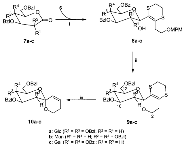
Scheme 2. Coupling and spirocyclization of sugars. i. THF, -78 °C; ii. BF 3 ·Et 2 O, CH 2 Cl 2 , room temp.; iii. Raney (Ni), THF, room temp.
