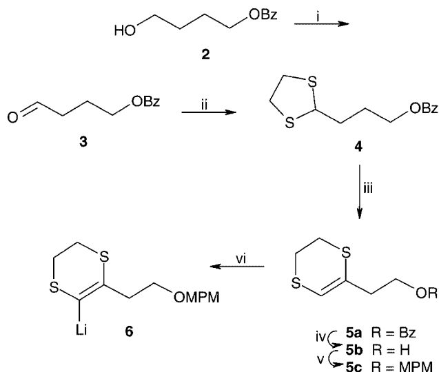
Scheme 1. Preparation of the lithiated reagent 6 . i. PCC, CH 2 Cl 2 , room temp.; ii. polymer-bound DPP / I 2 , ethanedithiol, MeCN, room temp.; iii. NBS, CHCl 3 , room temp.; iv. MeONa, MeOH, room temp.; v. NaH, MPMCl, DMF, room temp.; vi. BuLi, THF, -78 °C
